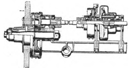
Winton Rear Axle Construction.
